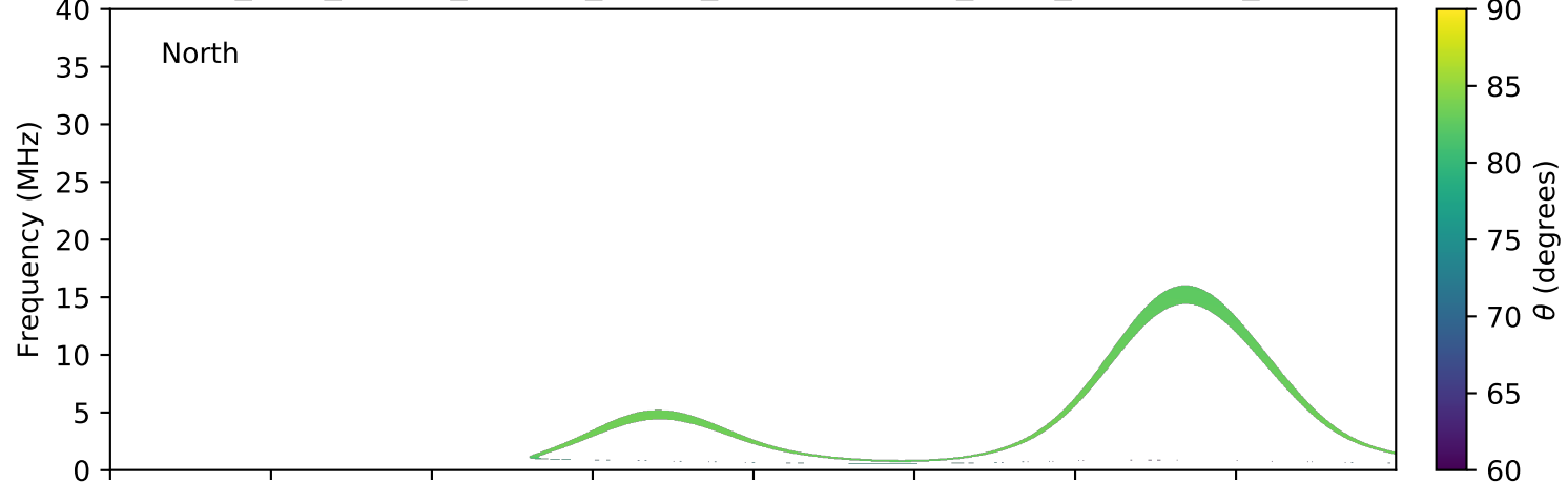
expres_juno_jupiter_europa_jrm09_lossc-wid1deg_3kev_20210802_v11.cdf
