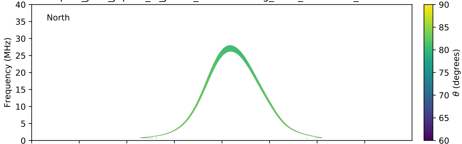
expres_juno_jupiter_io_jrm09_lossc-wid1deg_3kev_20210730_v11.cdf
