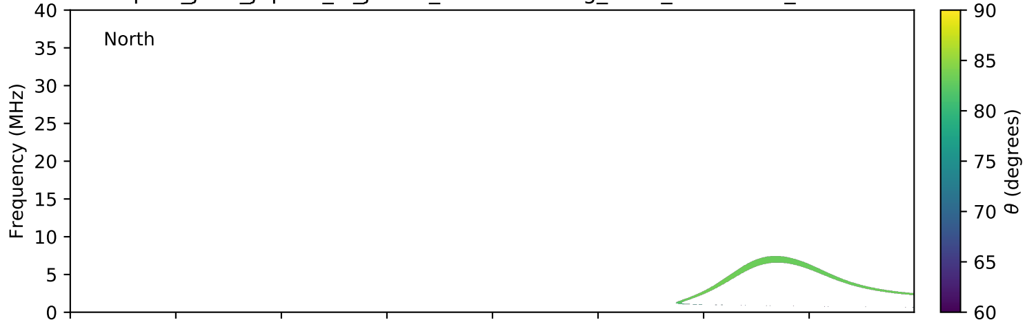
expres_juno_jupiter_io_jrm09_lossc-wid1deg_3kev_20210726_v11.cdf
