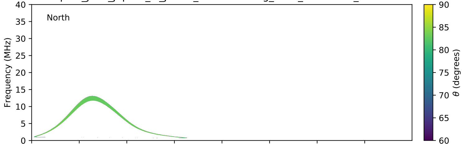
expres_juno_jupiter_io_jrm09_lossc-wid1deg_3kev_20210725_v11.cdf
