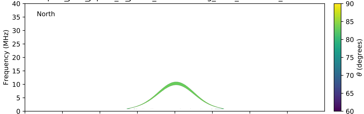
expres_juno_jupiter_io_jrm09_lossc-wid1deg_3kev_20210723_v11.cdf
