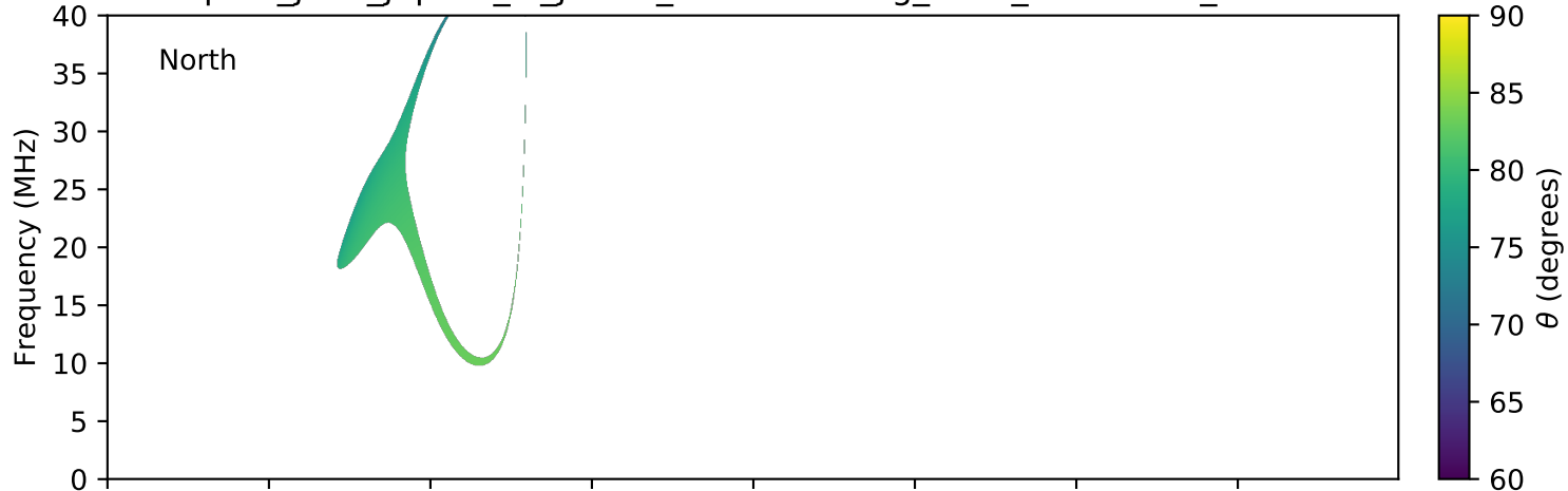
expres_juno_jupiter_io_jrm09_lossc-wid1deg_3kev_20210721_v11.cdf
