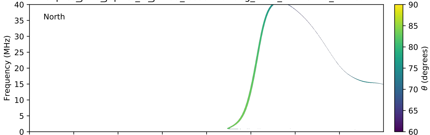
expres_juno_jupiter_io_jrm09_lossc-wid1deg_3kev_20210719_v11.cdf
