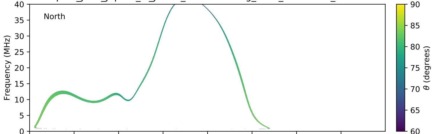
expres_juno_jupiter_io_jrm09_lossc-wid1deg_3kev_20210716_v11.cdf
