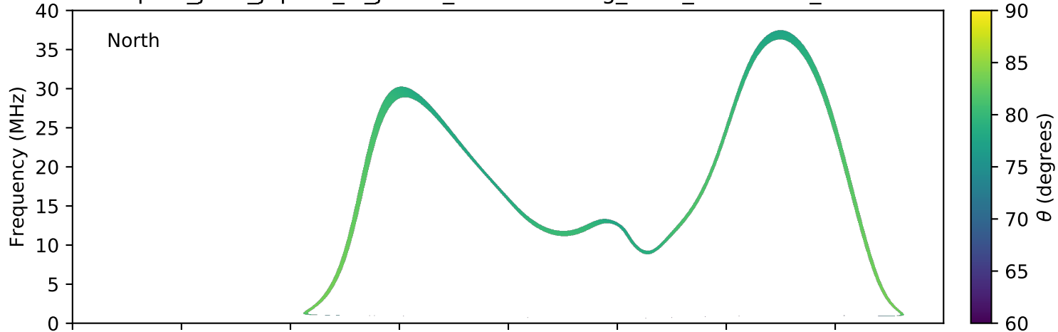
expres_juno_jupiter_io_jrm09_lossc-wid1deg_3kev_20210714_v11.cdf
