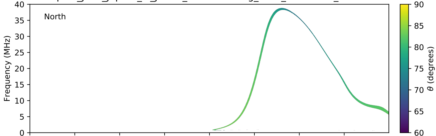
expres_juno_jupiter_io_jrm09_lossc-wid1deg_3kev_20210712_v11.cdf
