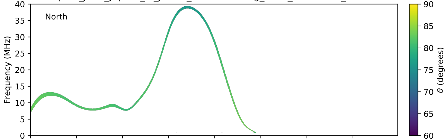
expres_juno_jupiter_io_jrm09_lossc-wid1deg_3kev_20210709_v11.cdf
