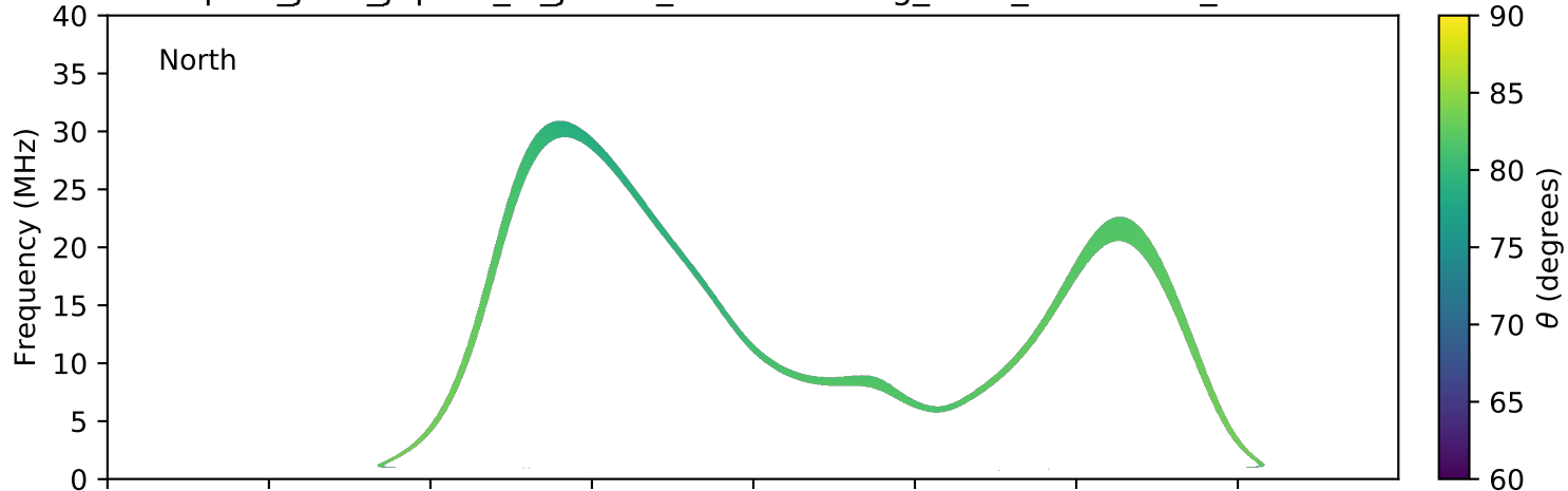
expres_juno_jupiter_io_jrm09_lossc-wid1deg_3kev_20210707_v11.cdf
