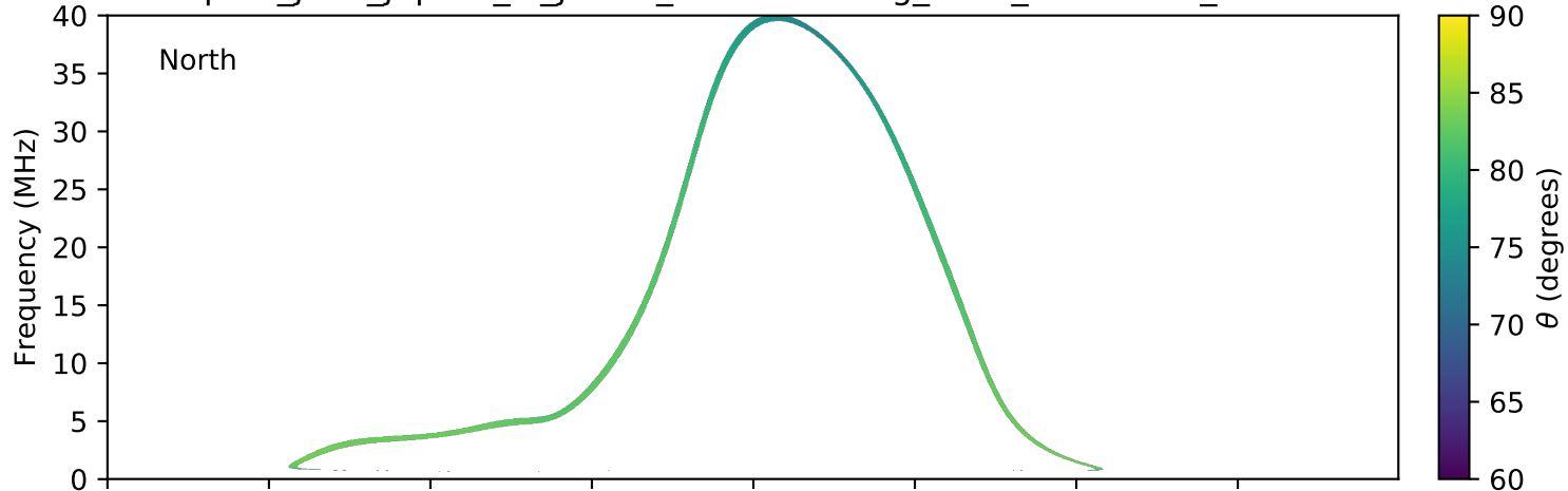
expres_juno_jupiter_io_jrm09_lossc-wid1deg_3kev_20210706_v11.cdf
