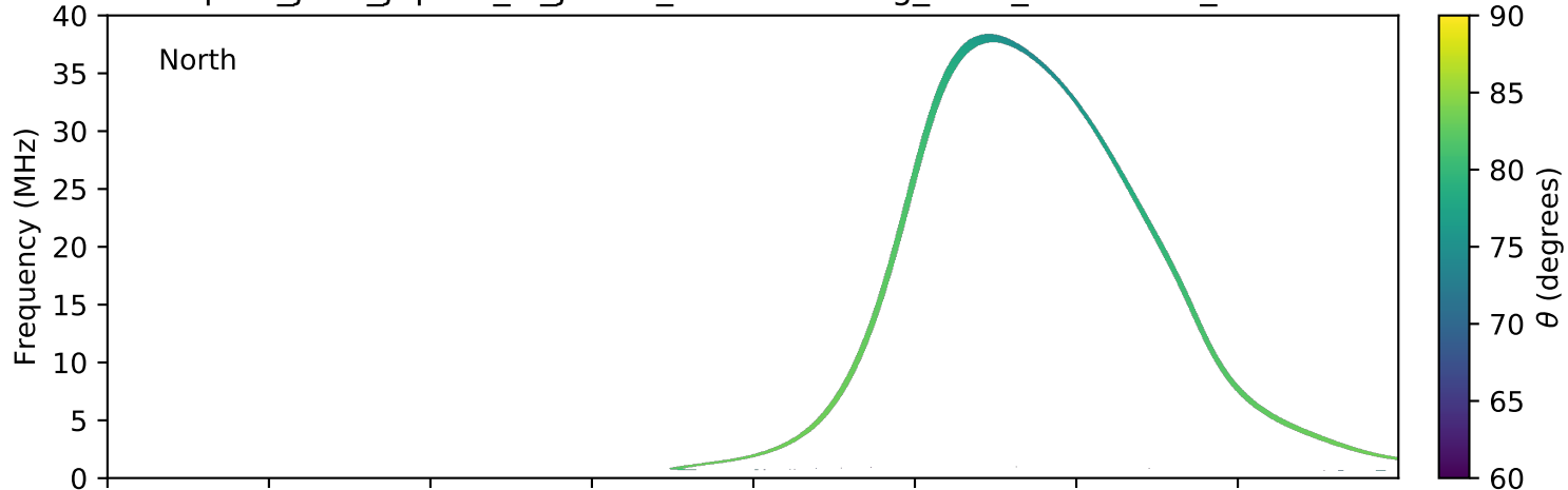
expres_juno_jupiter_io_jrm09_lossc-wid1deg_3kev_20210705_v11.cdf
