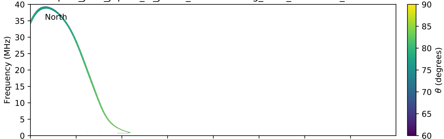
expres_juno_jupiter_io_jrm09_lossc-wid1deg_3kev_20210704_v11.cdf
