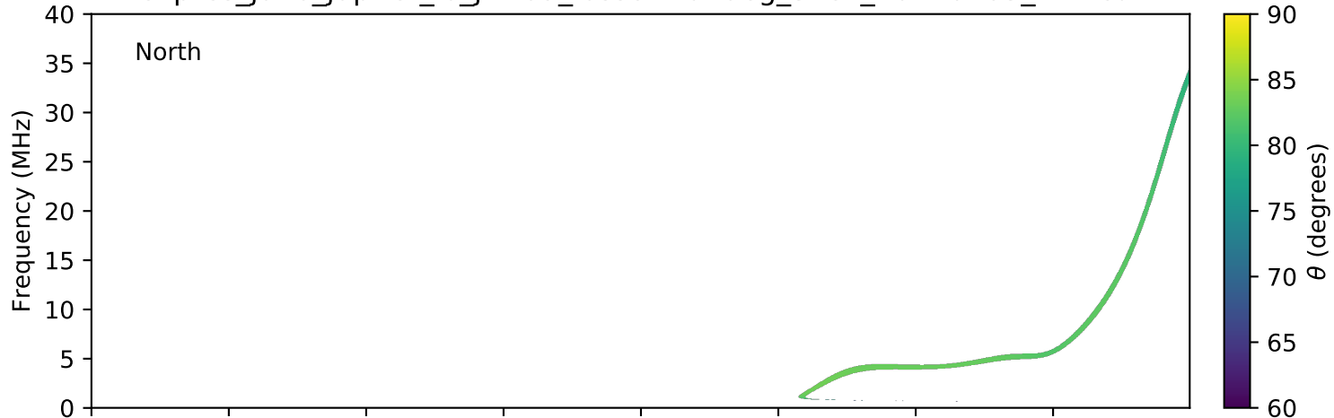
expres_juno_jupiter_io_jrm09_lossc-wid1deg_3kev_20210703_v11.cdf
