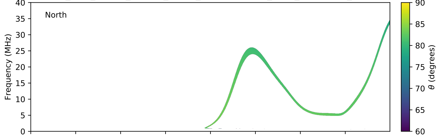
expres_juno_jupiter_europa_jrm09_lossc-wid1deg_3kev_20210715_v11.cdf
