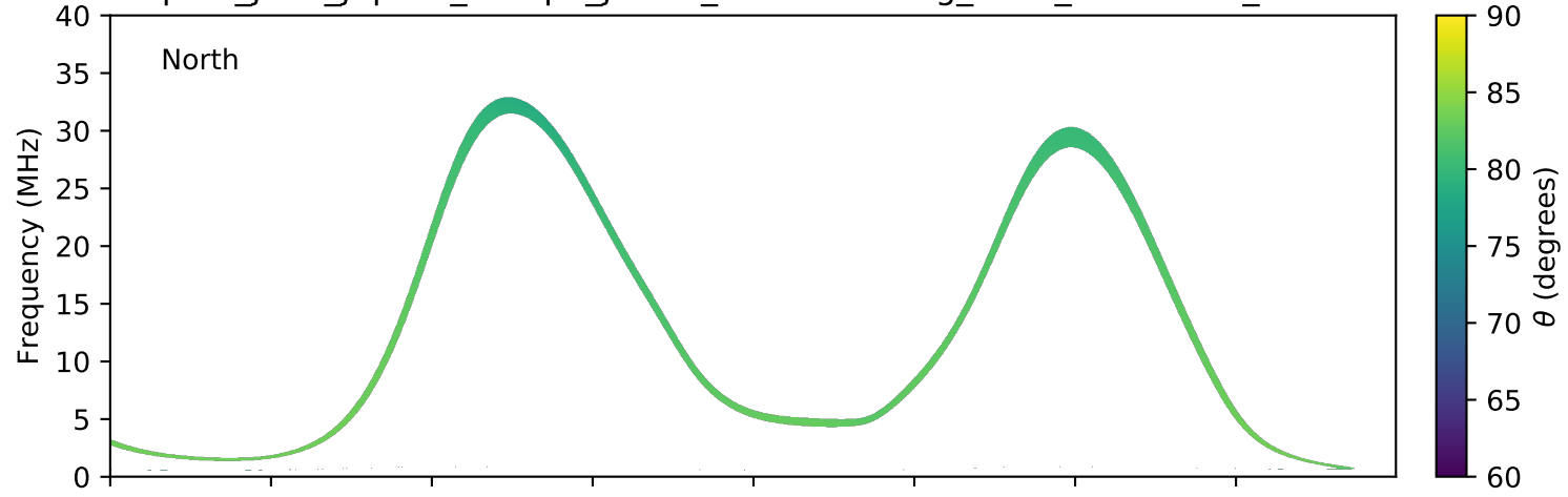
expres_juno_jupiter_europa_jrm09_lossc-wid1deg_3kev_20210712_v11.cdf
