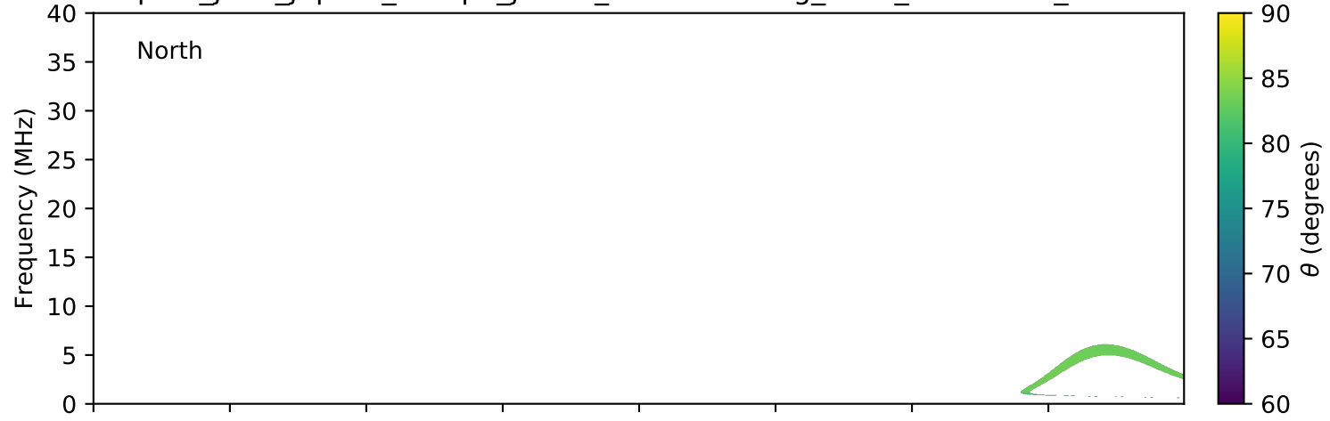
expres_juno_jupiter_europa_jrm09_lossc-wid1deg_3kev_20210711_v11.cdf
