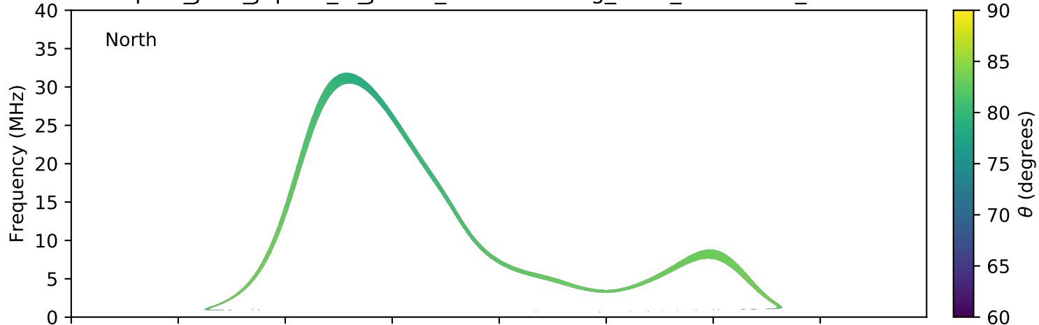
expres_juno_jupiter_io_jrm09_lossc-wid1deg_3kev_20210630_v11.cdf
