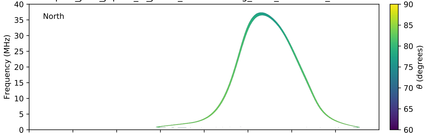
expres_juno_jupiter_io_jrm09_lossc-wid1deg_3kev_20210628_v11.cdf
