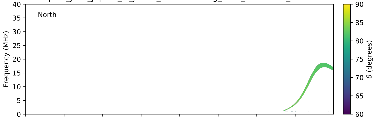
expres_juno_jupiter_io_jrm09_lossc-wid1deg_3kev_20210624_v11.cdf
