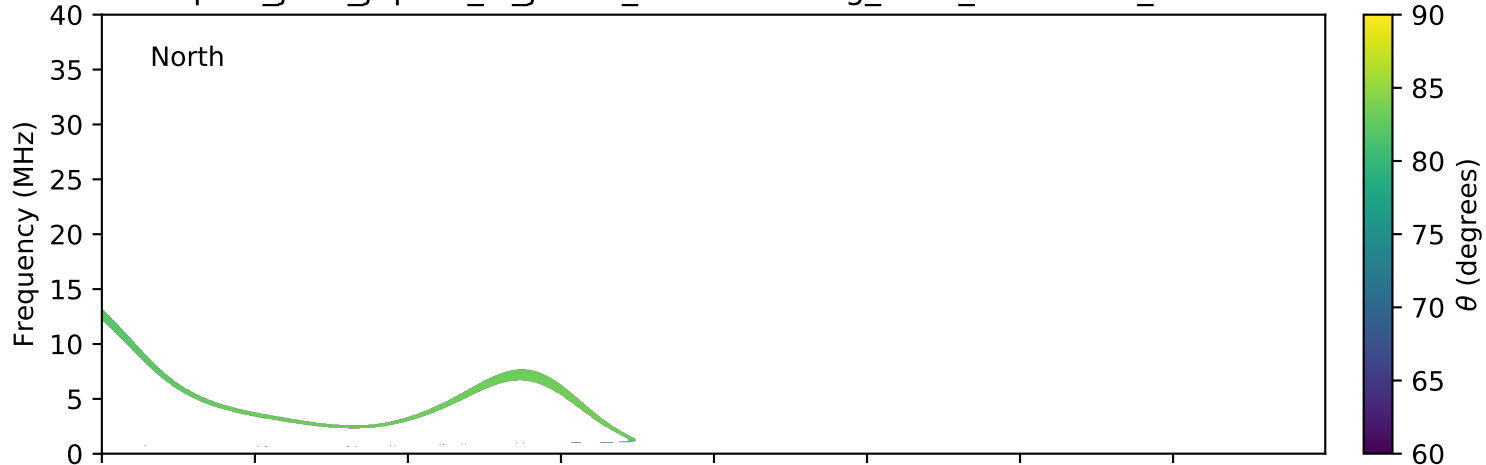
expres_juno_jupiter_io_jrm09_lossc-wid1deg_3kev_20210618_v11.cdf
