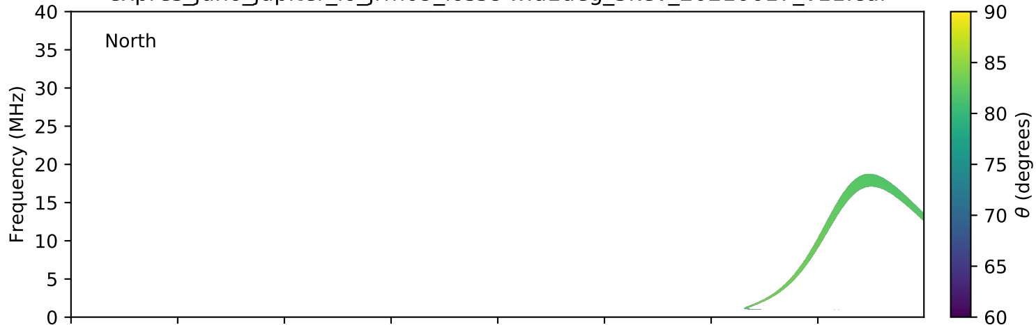
expres_juno_jupiter_io_jrm09_lossc-wid1deg_3kev_20210617_v11.cdf
