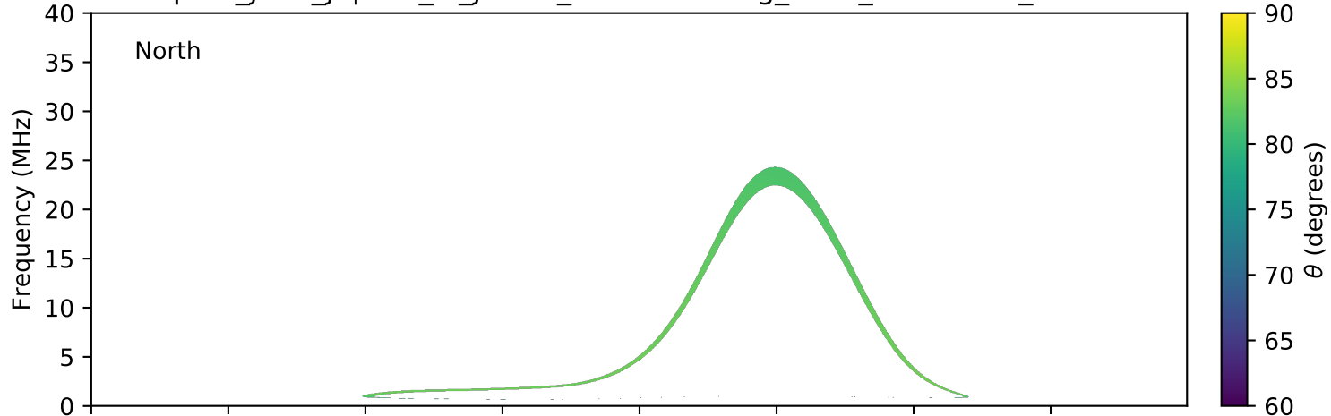
expres_juno_jupiter_io_jrm09_lossc-wid1deg_3kev_20210614_v11.cdf
