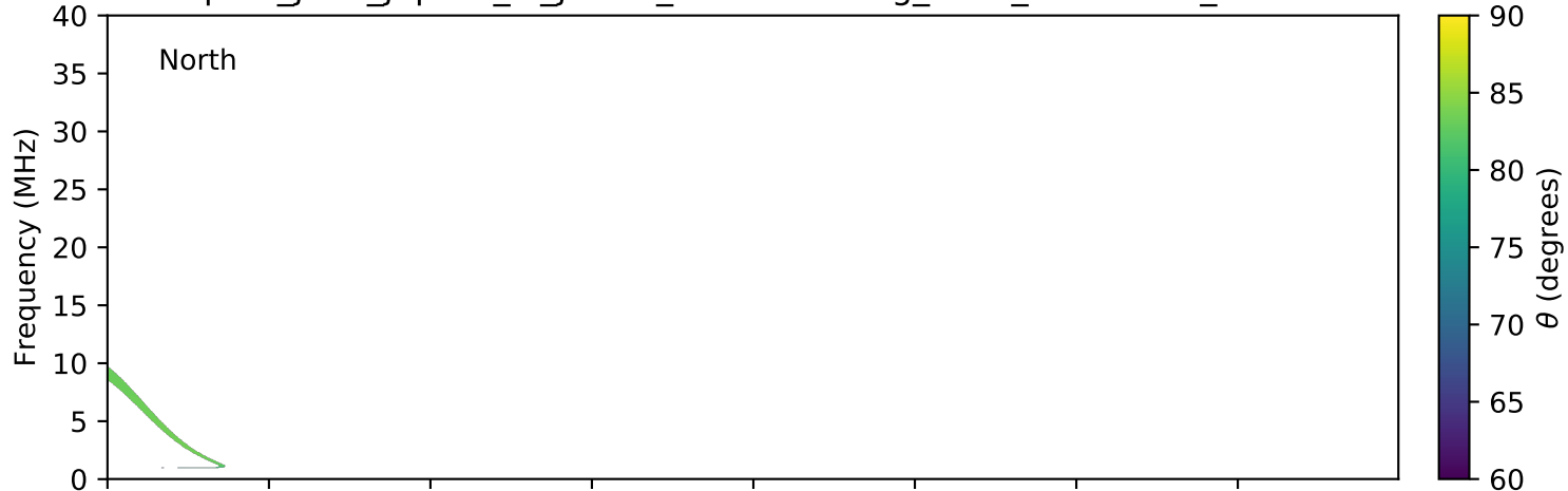
expres_juno_jupiter_io_jrm09_lossc-wid1deg_3kev_20210613_v11.cdf
