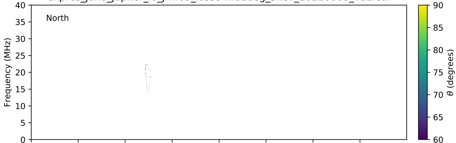
expres_juno_jupiter_io_jrm09_lossc-wid1deg_3kev_20210608_v11.cdf
