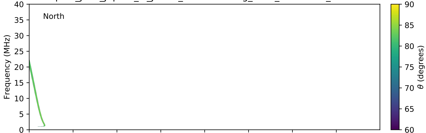
expres_juno_jupiter_io_jrm09_lossc-wid1deg_3kev_20210606_v11.cdf
