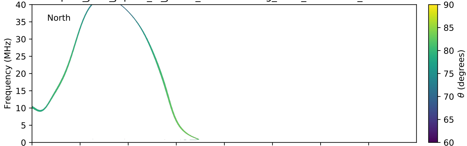
expres_juno_jupiter_io_jrm09_lossc-wid1deg_3kev_20210602_v11.cdf
