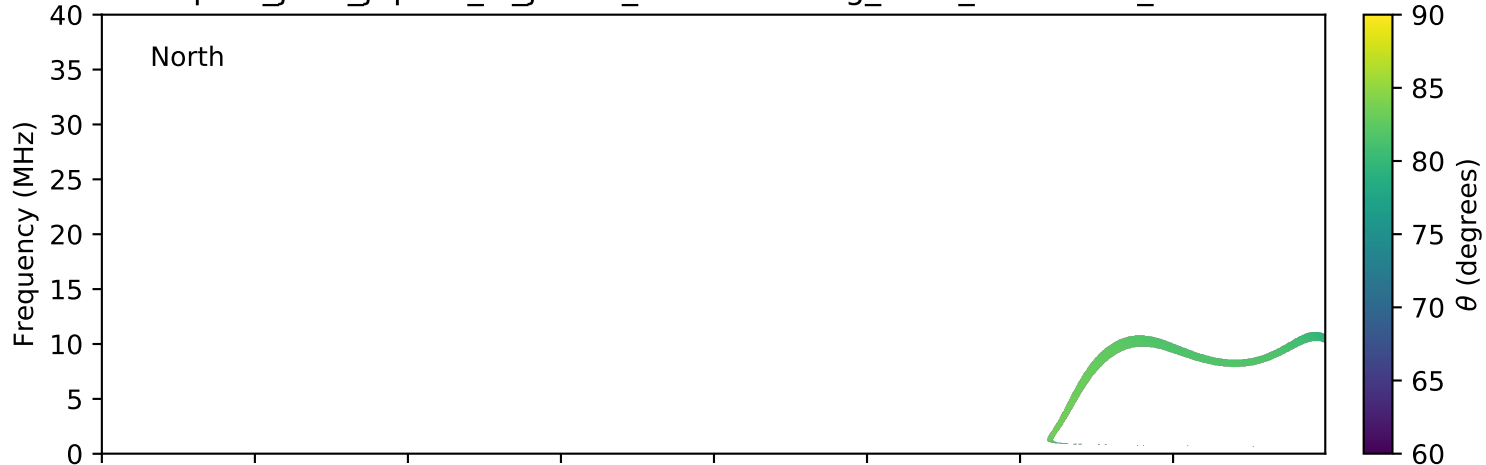
expres_juno_jupiter_io_jrm09_lossc-wid1deg_3kev_20210601_v11.cdf
