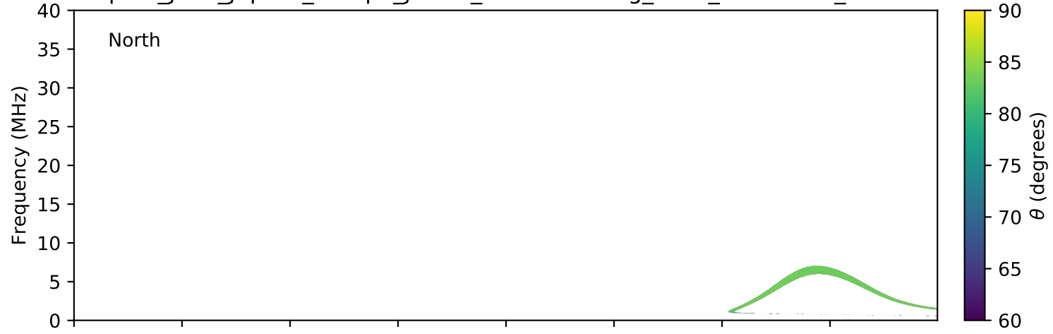
expres_juno_jupiter_europa_jrm09_lossc-wid1deg_3kev_20210627_v11.cdf
