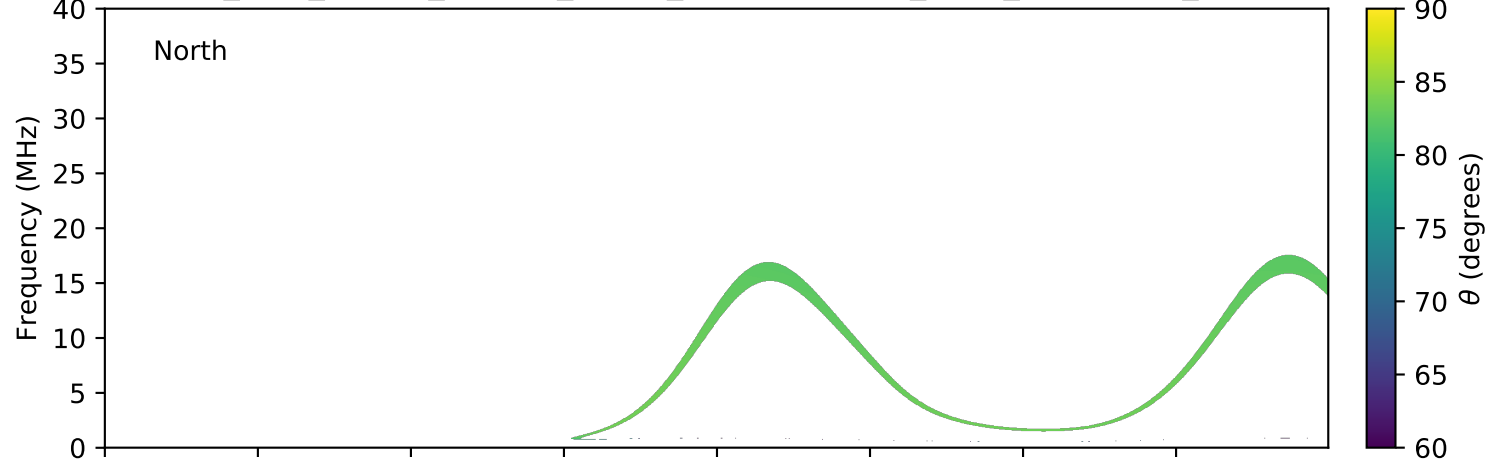
expres_juno_jupiter_europa_jrm09_lossc-wid1deg_3kev_20210624_v11.cdf
