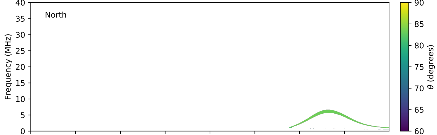
expres_juno_jupiter_europa_jrm09_lossc-wid1deg_3kev_20210620_v11.cdf
