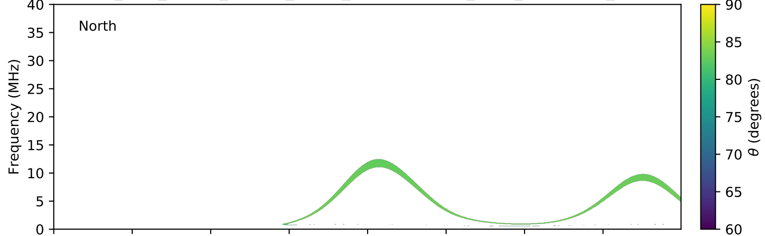
expres_juno_jupiter_europa_jrm09_lossc-wid1deg_3kev_20210617_v11.cdf
