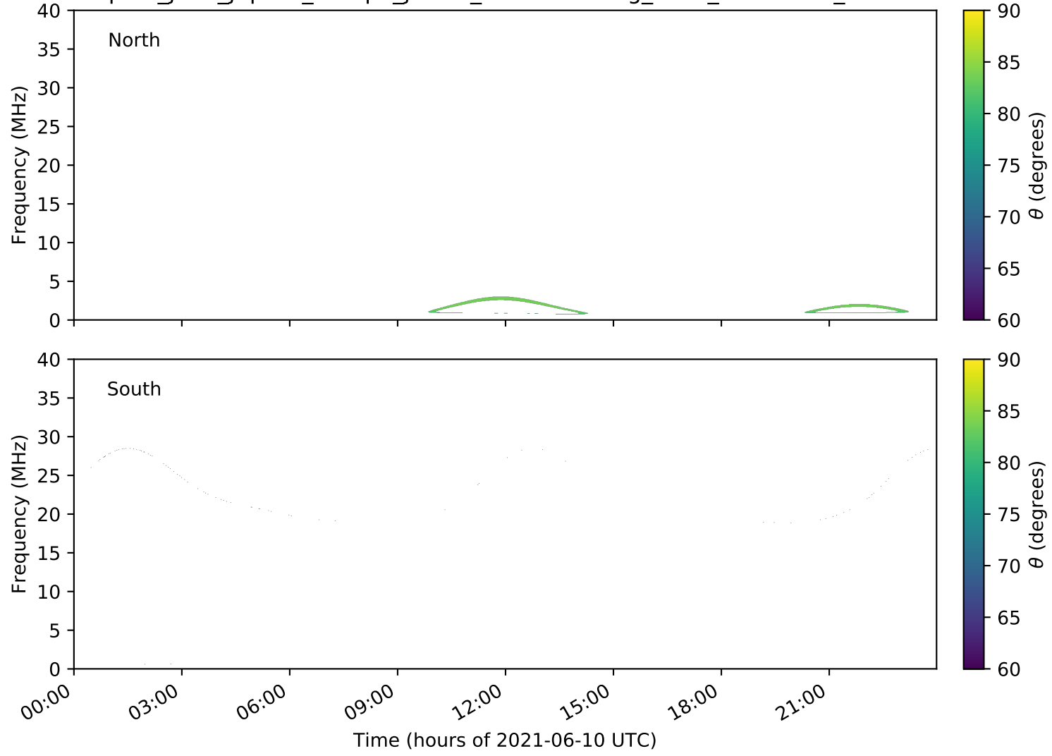
expres_juno_jupiter_europa_jrm09_lossc-wid1deg_3kev_20210610_v11.cdf
