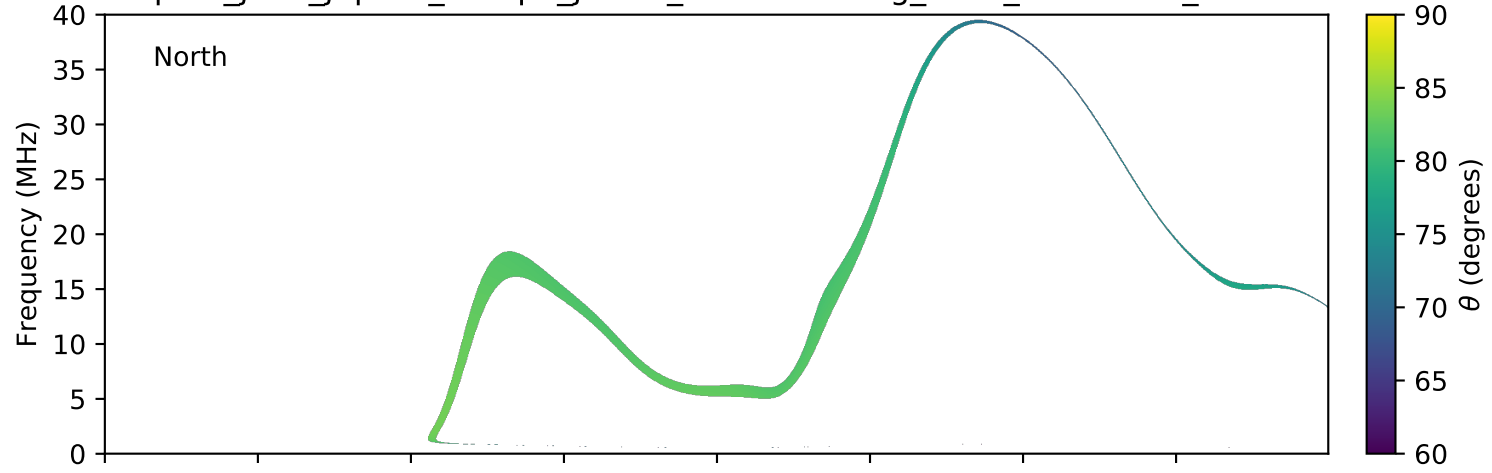
expres_juno_jupiter_europa_jrm09_lossc-wid1deg_3kev_20210606_v11.cdf
