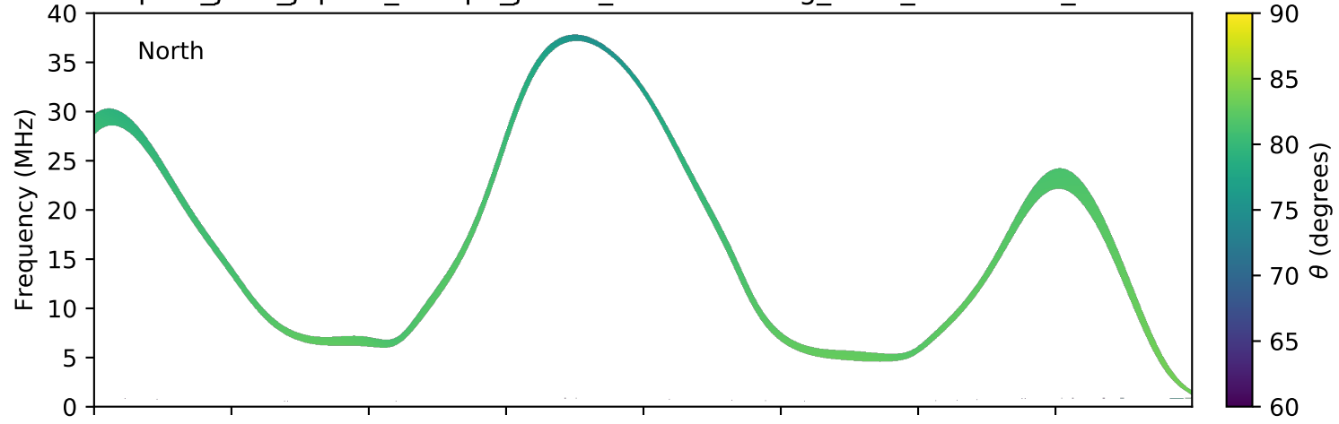
expres_juno_jupiter_europa_jrm09_lossc-wid1deg_3kev_20210603_v11.cdf
