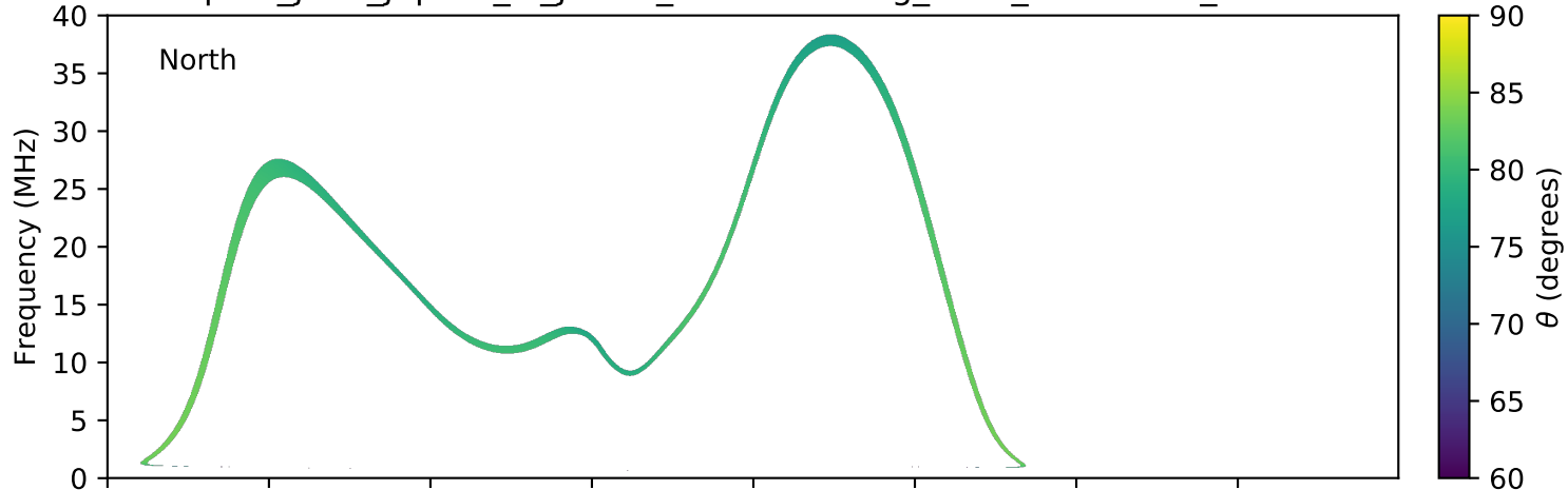
expres_juno_jupiter_io_jrm09_lossc-wid1deg_3kev_20210531_v11.cdf
