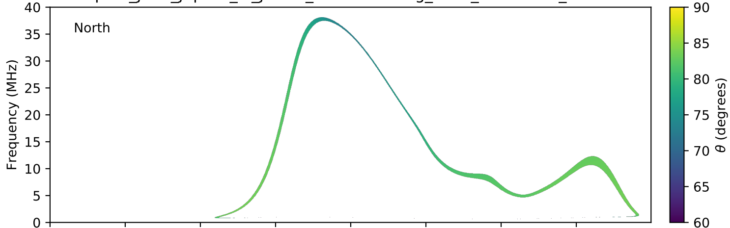
expres_juno_jupiter_io_jrm09_lossc-wid1deg_3kev_20210529_v11.cdf
