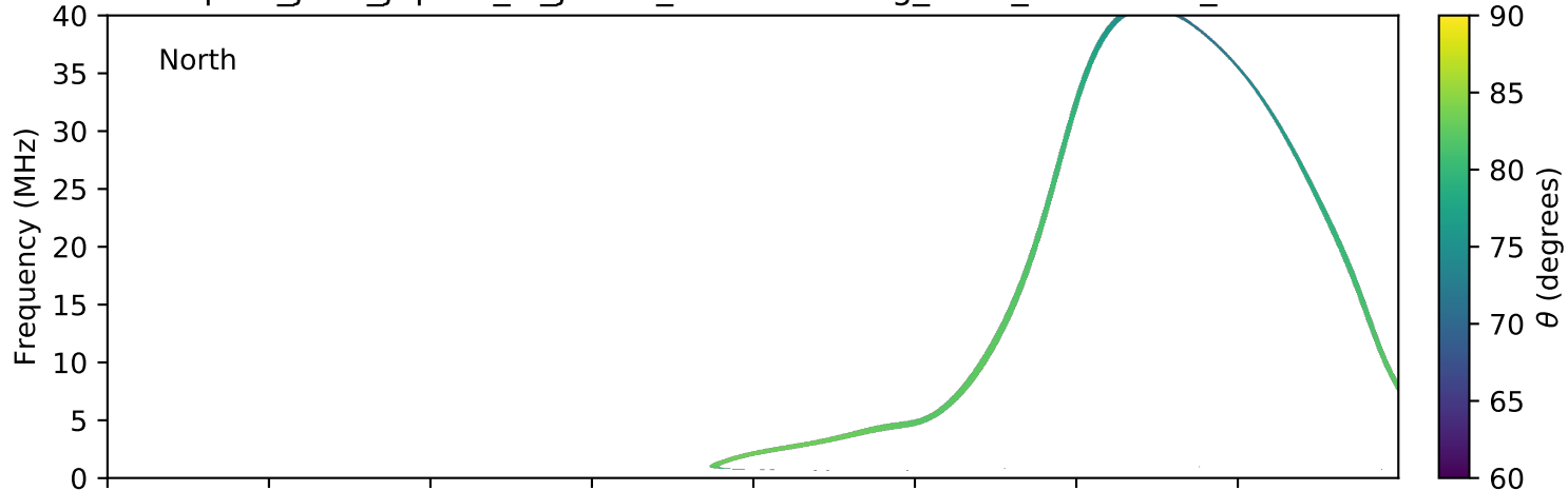
expres_juno_jupiter_io_jrm09_lossc-wid1deg_3kev_20210527_v11.cdf
