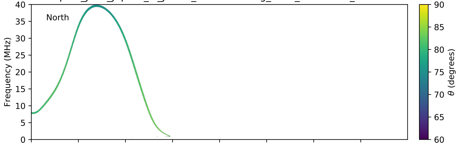
expres_juno_jupiter_io_jrm09_lossc-wid1deg_3kev_20210526_v11.cdf
