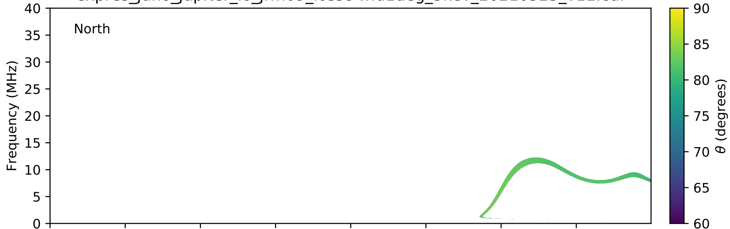
expres_juno_jupiter_io_jrm09_lossc-wid1deg_3kev_20210525_v11.cdf
