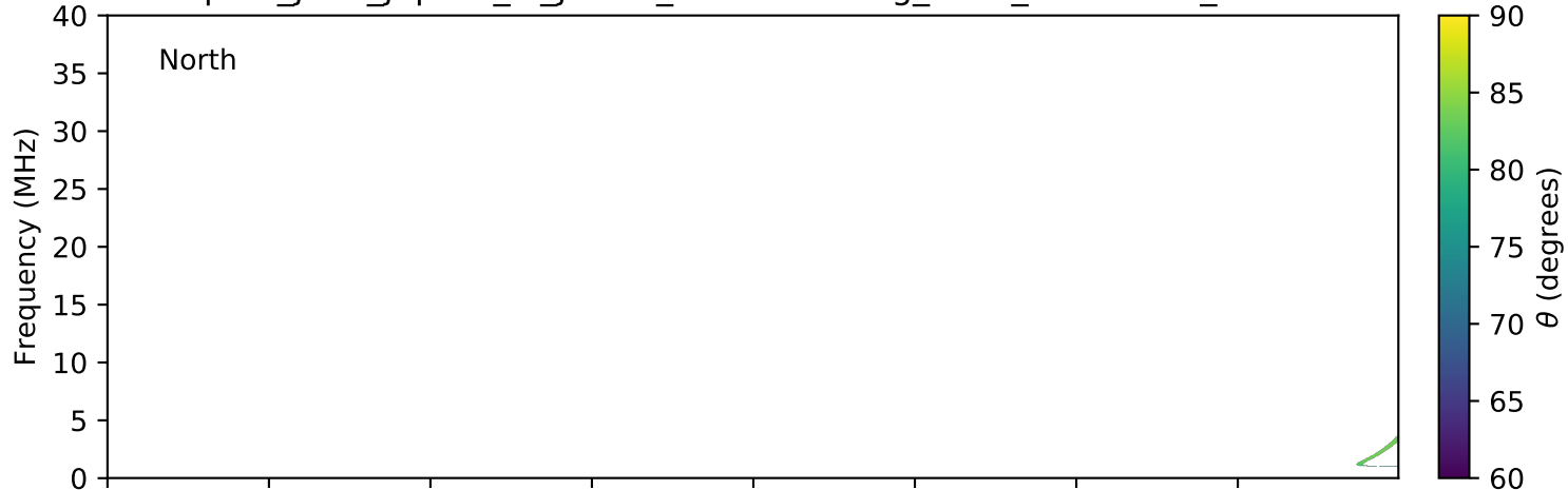
expres_juno_jupiter_io_jrm09_lossc-wid1deg_3kev_20210523_v11.cdf
