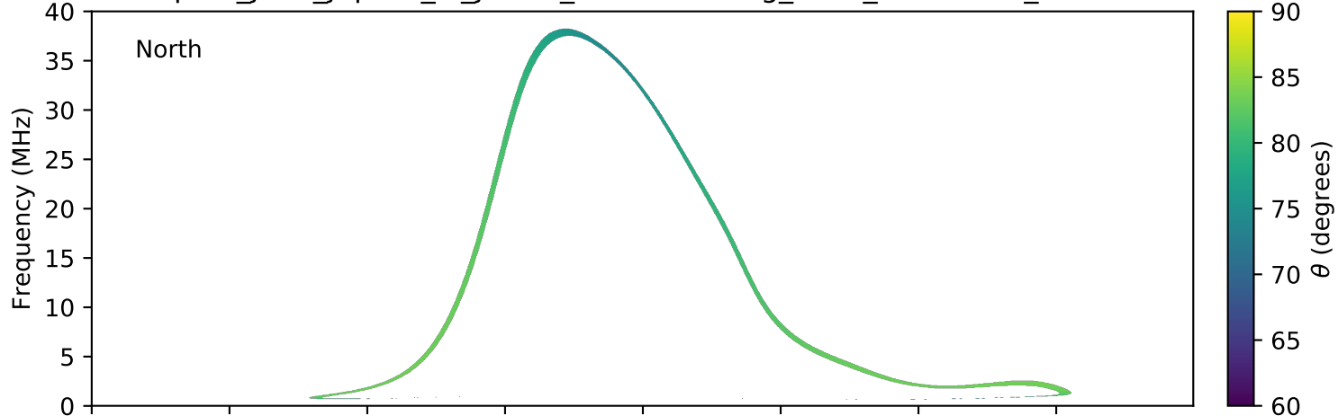
expres_juno_jupiter_io_jrm09_lossc-wid1deg_3kev_20210522_v11.cdf
