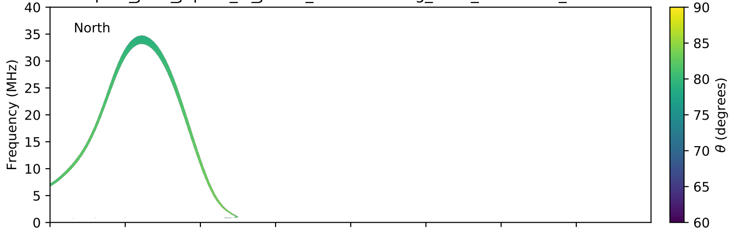
expres_juno_jupiter_io_jrm09_lossc-wid1deg_3kev_20210519_v11.cdf
