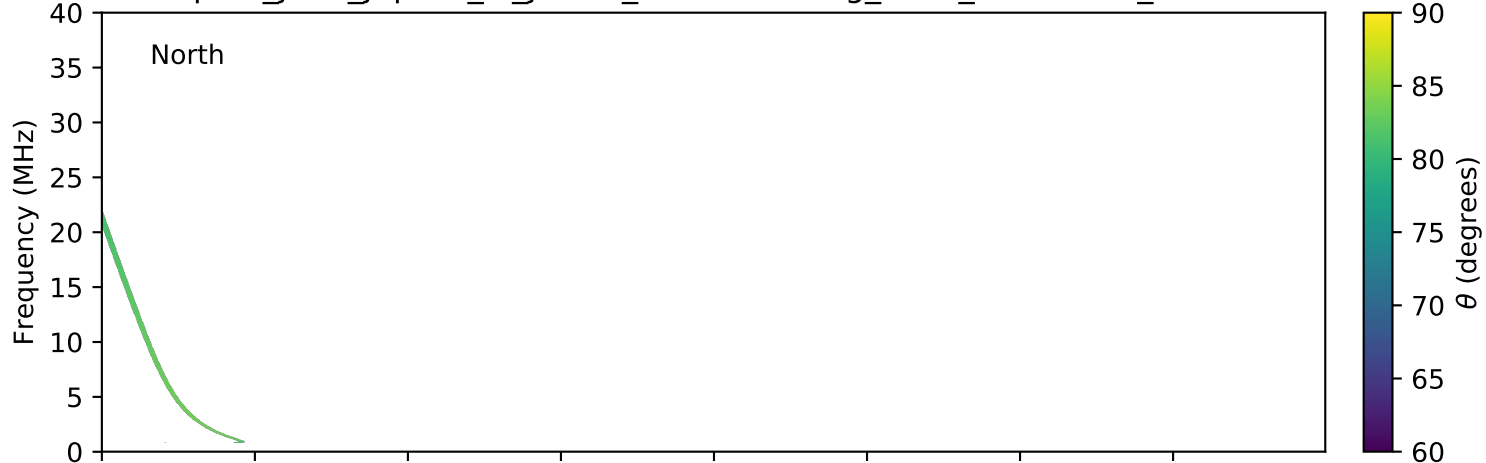
expres_juno_jupiter_io_jrm09_lossc-wid1deg_3kev_20210518_v11.cdf
