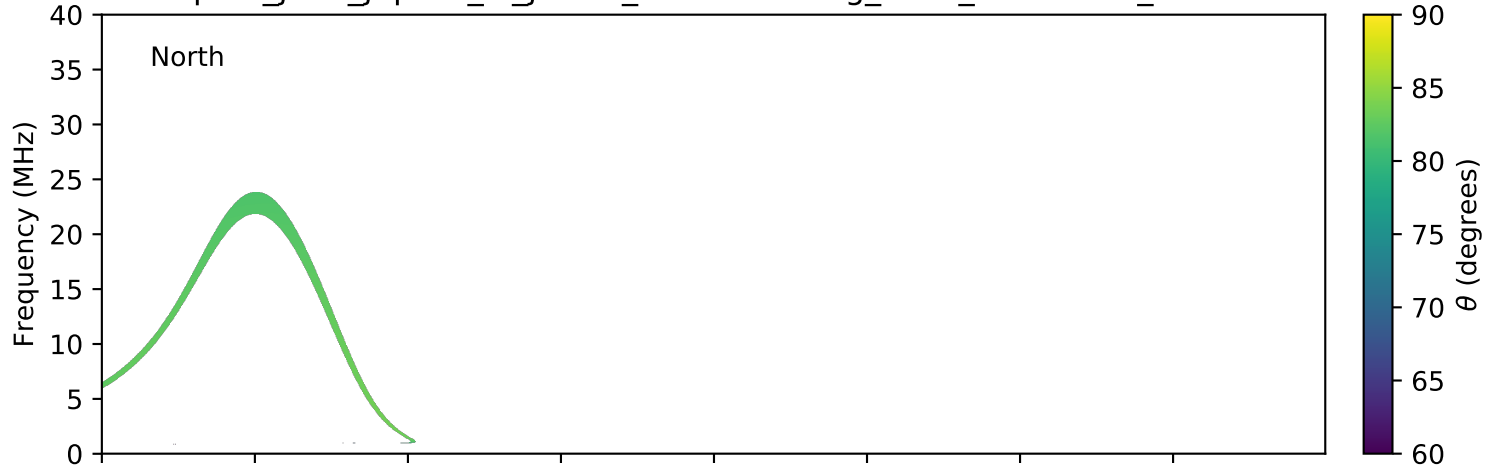
expres_juno_jupiter_io_jrm09_lossc-wid1deg_3kev_20210512_v11.cdf
