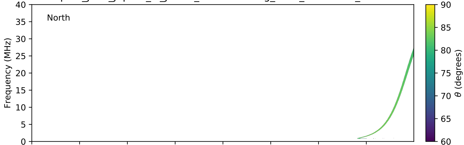
expres_juno_jupiter_io_jrm09_lossc-wid1deg_3kev_20210509_v11.cdf
