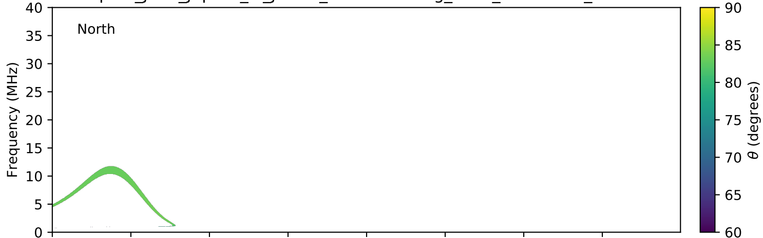
expres_juno_jupiter_io_jrm09_lossc-wid1deg_3kev_20210505_v11.cdf
