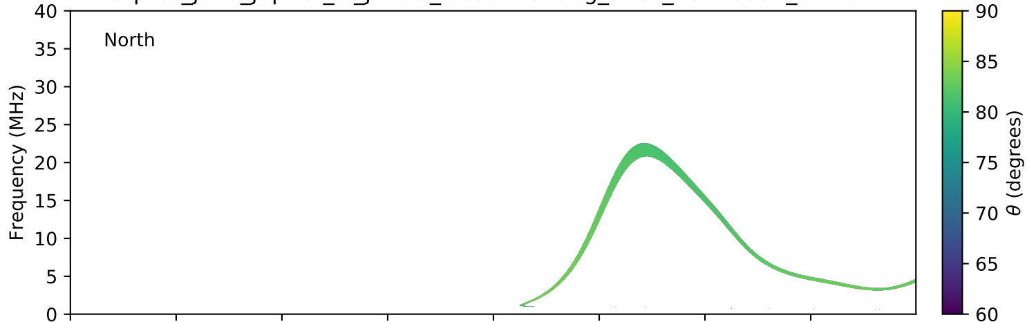
expres_juno_jupiter_io_jrm09_lossc-wid1deg_3kev_20210504_v11.cdf
